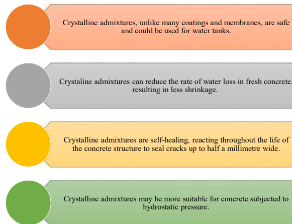
Fig. 11. Advantages of crystalline admixtures against other waterproofing admixtures.
